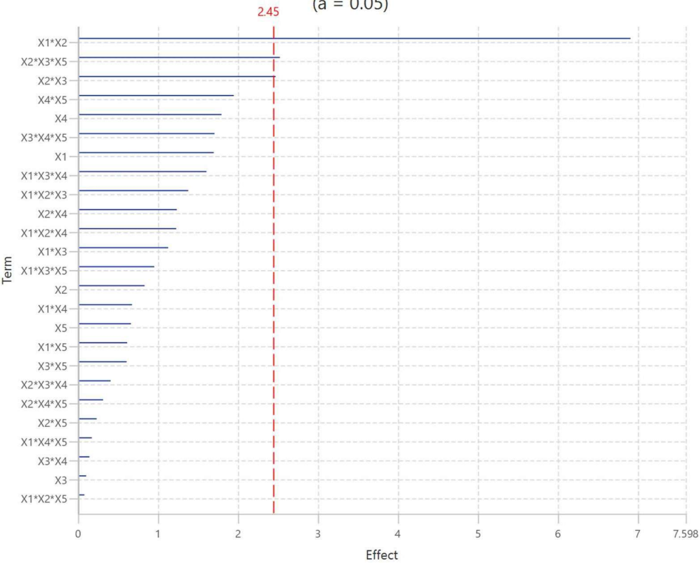
Pareto Chart for Standardized Effects: Y 2 (a = 0.05)
